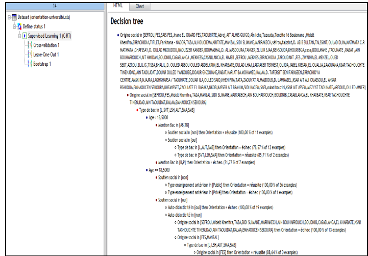
Fig. 4. Resulting predictive model of learning.
