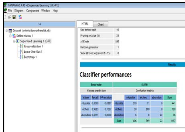
Fig. 3. Confusion matrix on the training sample.
